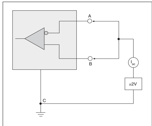
Figure 8. V.35 Receiver Input Short-Circuit Impedance
